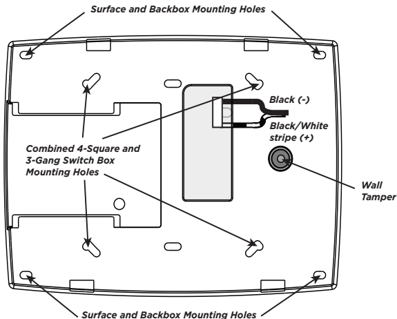
Figure 3: Mounting Holes on Keypad Back
