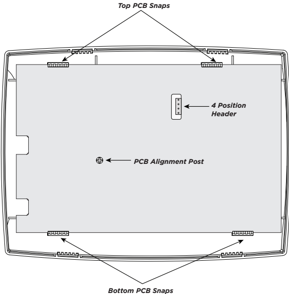
Figure 9: PCB Snaps
