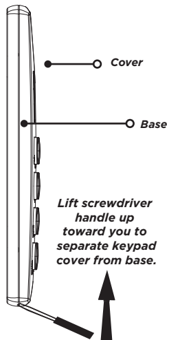
Figure 2: Separate the Keypad Housing
